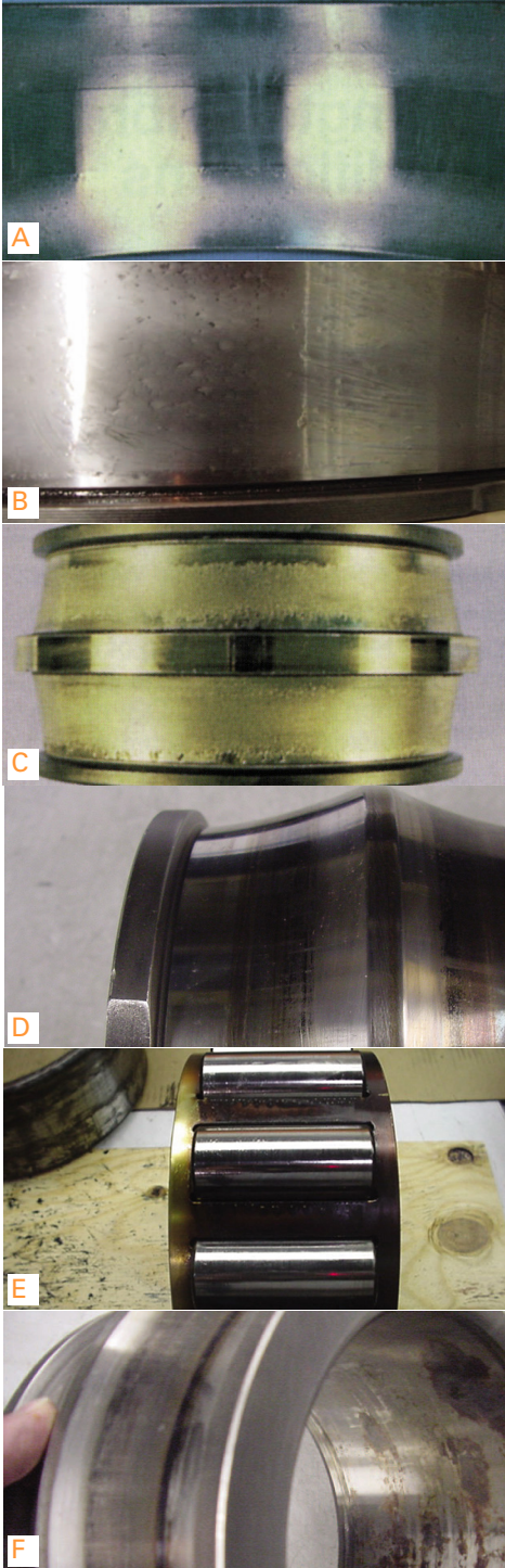
Figure 3: Common bearing damage modes
