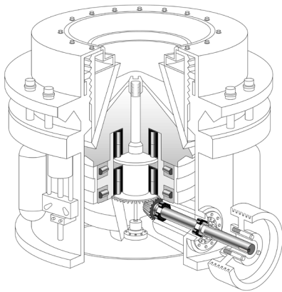
Figure 2: Cylindrical, tapered, thrust and plain bearings are all commonly found in a cone crusher.
